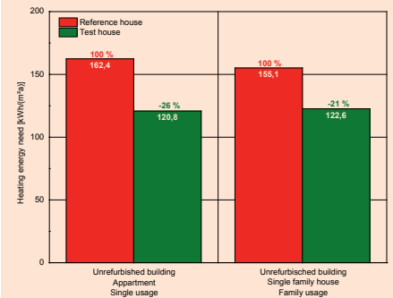
Fig. 1: Net heating energy savings for an unrefurbished apartment occupied by a single and for a single family house, occupied by a family.
